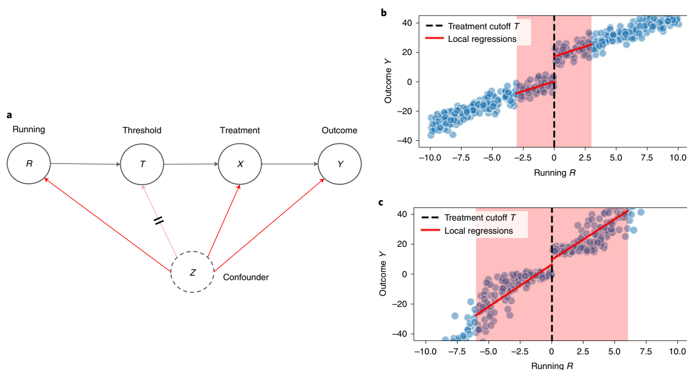
Fig. 3 | DAG and plots of RDDs. a , Graphical depiction of how RDDs use a threshold T in a continuous running variable R to effectively randomize treatment X (crossed red line) to estimate causal effects Y . b , Scatterplot (blue dots) and fitted local regressions (red lines) within the bandwidth (shaded red regions) of outcome Y on running variable R for simulated linear data to the left and right of the cutoff (dashed line). c , Scatterplot (blue dots) and fitted local regressions (red lines) within the bandwidth (shaded red regions) of outcome Y on running variable R for simulated nonlinear data to the left and right of the cutoff (dashed line).
