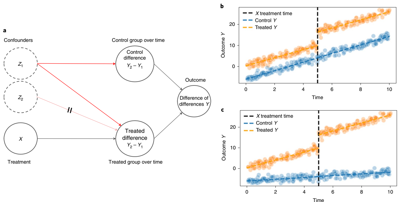
Fig. 4 | DAG and plots of DiD. a , Graphical representation of DiD, where both the control and treated groups are affected by the confounder Z_1 , but the difference of their differences pre- and post-treatment yield unbiased estimates of the outcome Y . An appropriate control group must be chosen such that any confounders affect both groups (the crossed edge of Z_2 affecting only the treated group would be a violation of this). b , Scatterplot of outcomes Y for both the treated group (orange) and the control group (blue) over time in simulated data where parallel trends holds, with a treatment X being applied (dashed) to the treated group. c , Scatterplot of outcomes Y for both the treated group (orange) and the control group (blue) over time in simulated data where the parallel trends assumption is violated.
